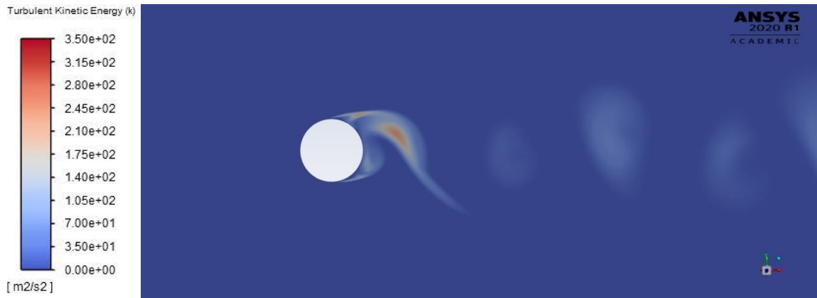
Figure 3.17: Turbulent kinetic energy contour plot ( \Delta t=1 \cdot 10^{-5} s)
