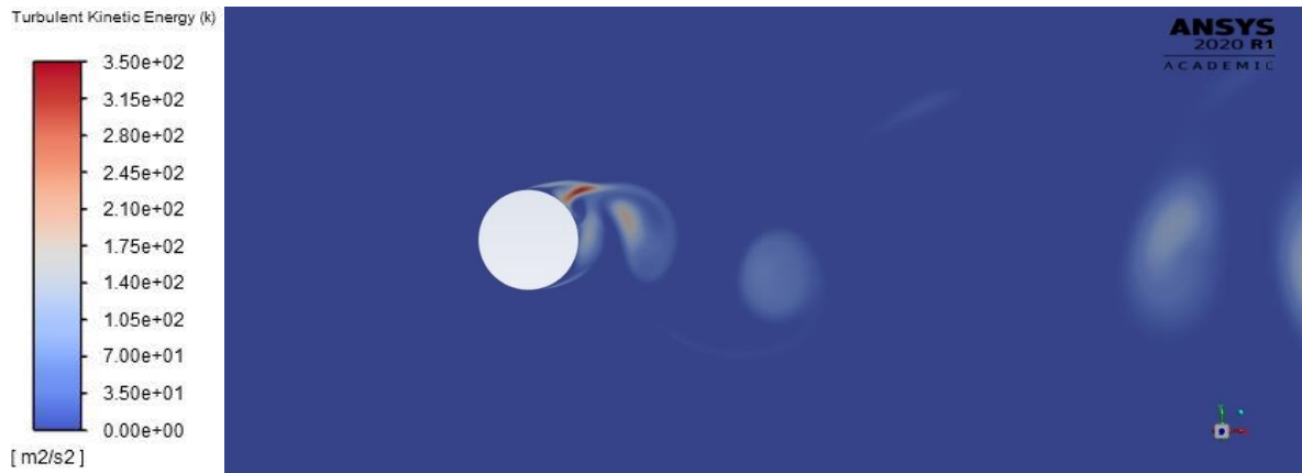
Figure 3.23: Turbulent kinetic energy contour plot ( \Delta t=1 \cdot 10^{-6} s)
