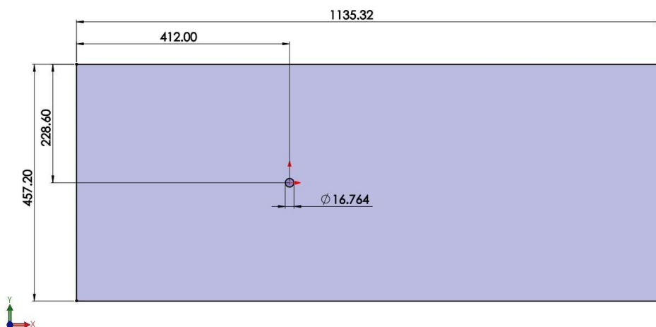
Figure 3.1: 2-D geometry
