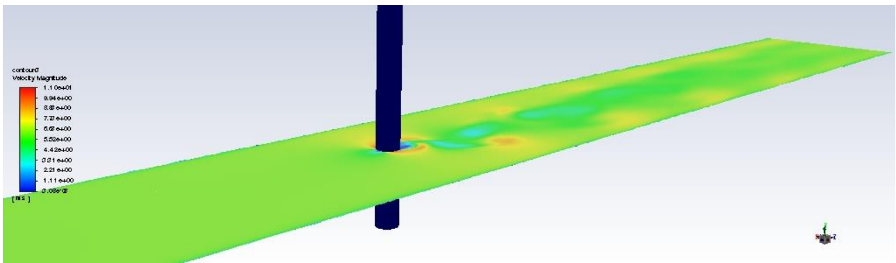
Figure 4.61: Velocity magnitude contours at t=0.8625 s
