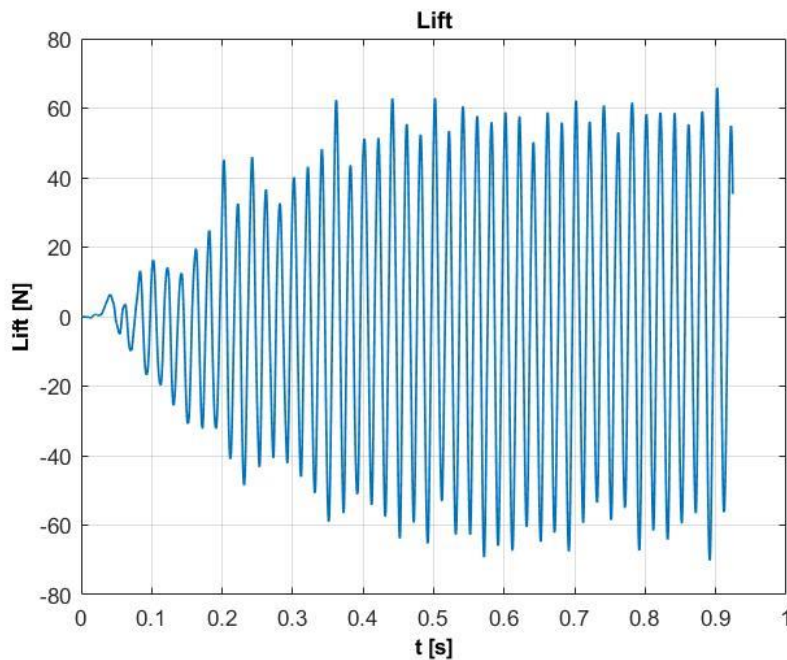
Figure 4.65: Temporal evolution of the lift on the thermowell
