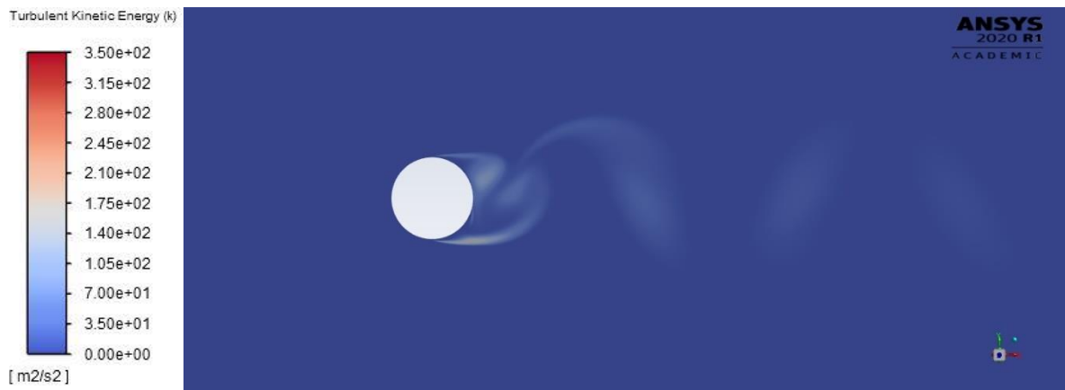
Figure 3.14: Turbulent kinetic energy contour plot ( \Delta t=5 \cdot 10^{-5} s)
