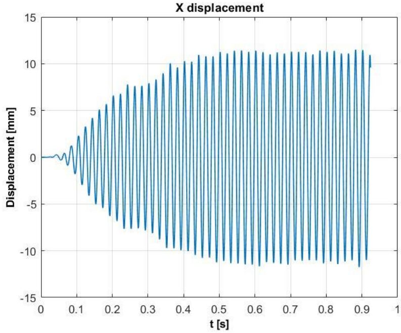
Figure 4.57: Transverse tip displacement, \zeta=0.041
