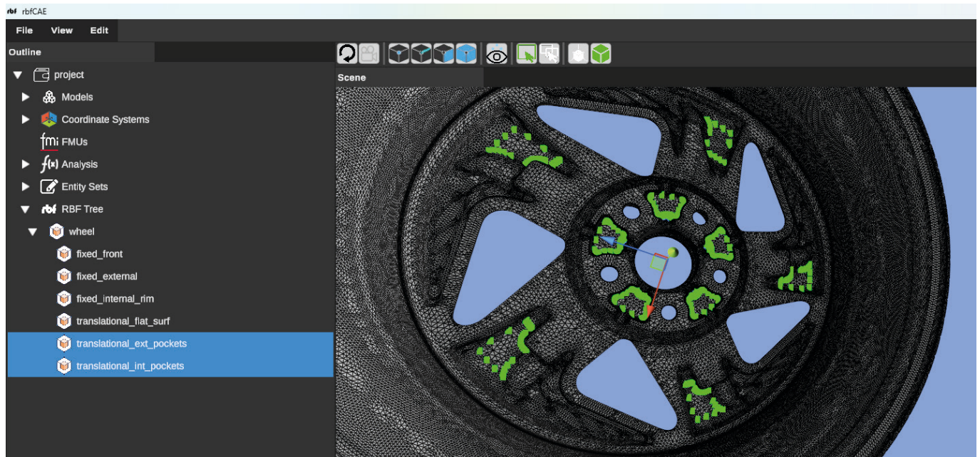
Fig. 3. rbfCAE platform setup for parametric mesh morphing.
